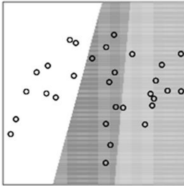
Figure 1. Partition from linear discriminant analysis.
