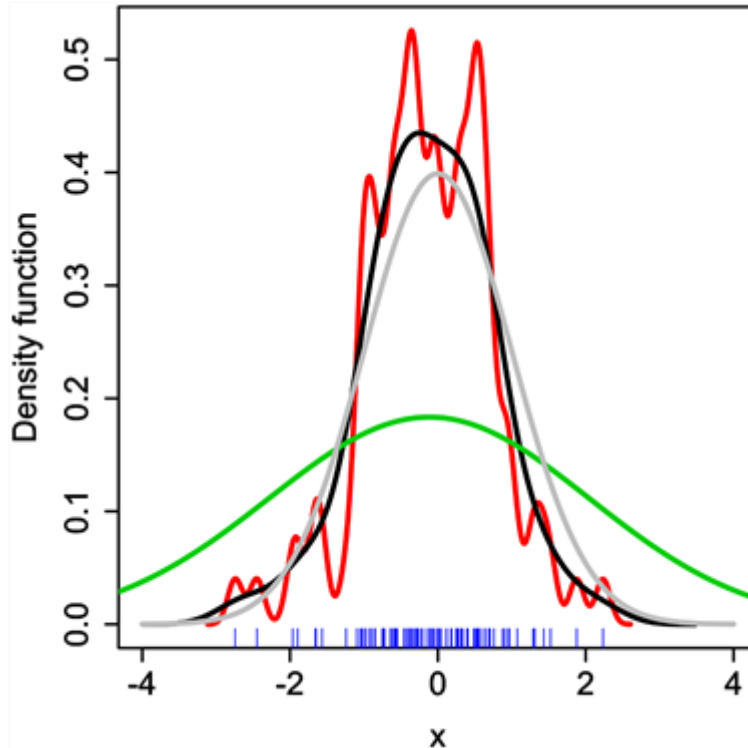
Figure 4. Kernel Density Estimate (KDE) with different bandwidths of a random sample.
