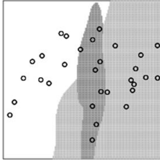
Figure 3. Partition from kernel discriminant analysis.
