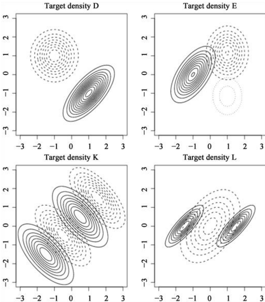
Figure 5. Contour plots for the target densities D, E, K, L for discriminant analysers: solid contours- \pi_1 f_1 , dashed lines- \pi_2 f_2 and dotted lines- \pi_3 f_3 .
