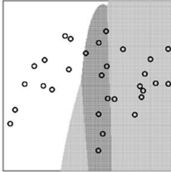
Figure 2. Partition from quadratic discriminant analysis.
